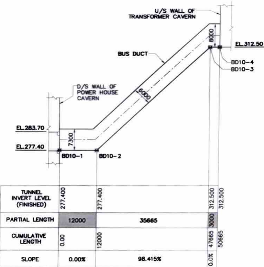
SECTION 4004/1000
