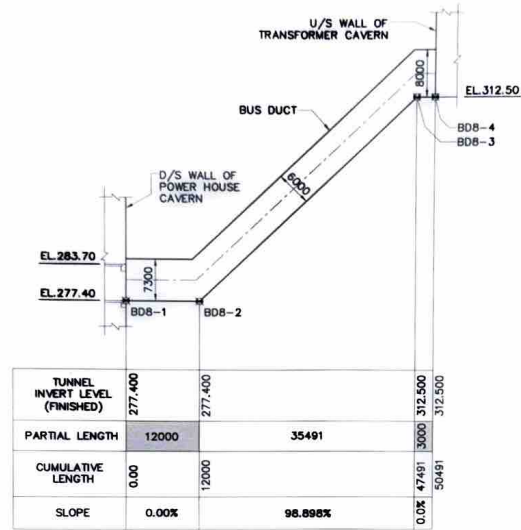
SECTION 4004/1000
