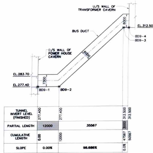
SECTION 4004/1000
