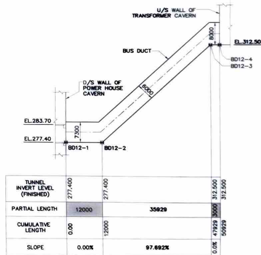
SECTION 4004/1000
